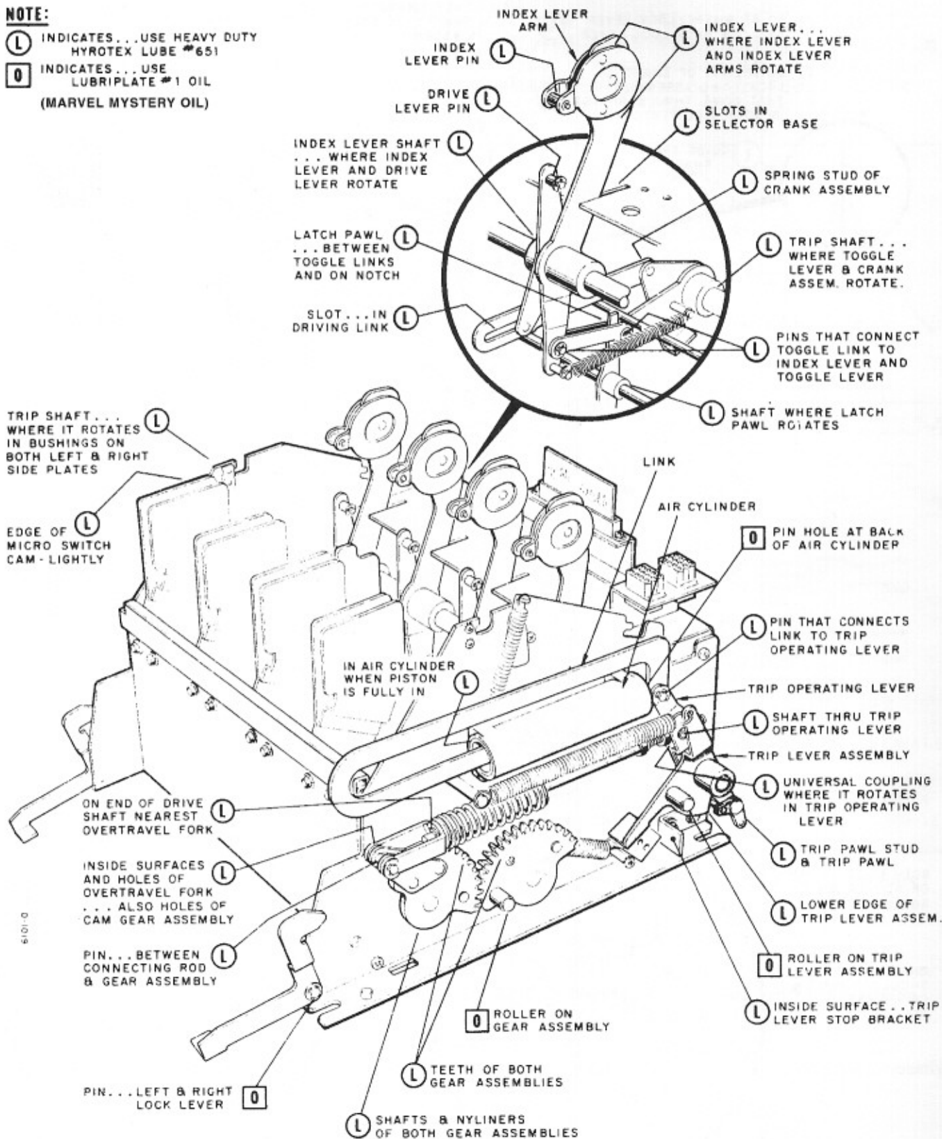
Figure 12. Reel Mechanism - (Soft Cushion)
