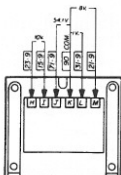
SECONDARY TRANSFORMER WIRING 120V, 50/60Hz.
