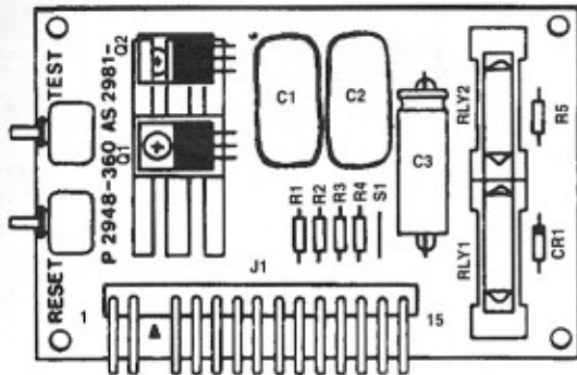
AS-2981-4 HOPPER CONTROL BOARD ASSEMBLY
